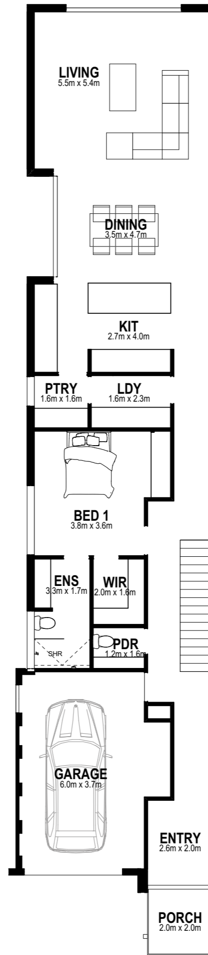
Ground Floor
