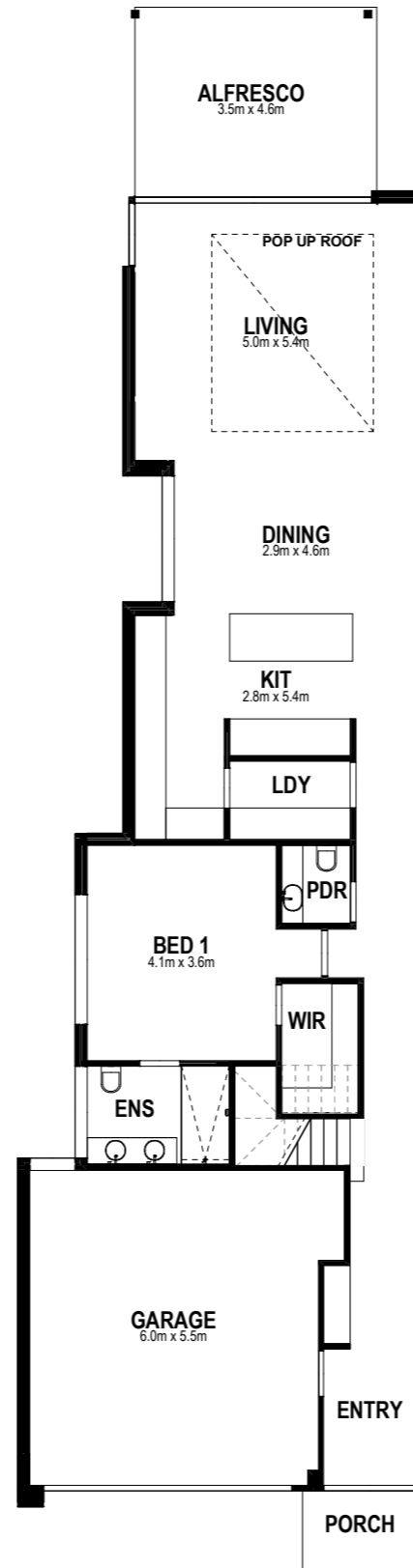
First Floor
