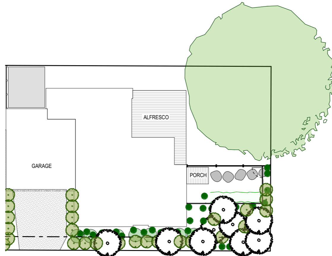
Site Plan
